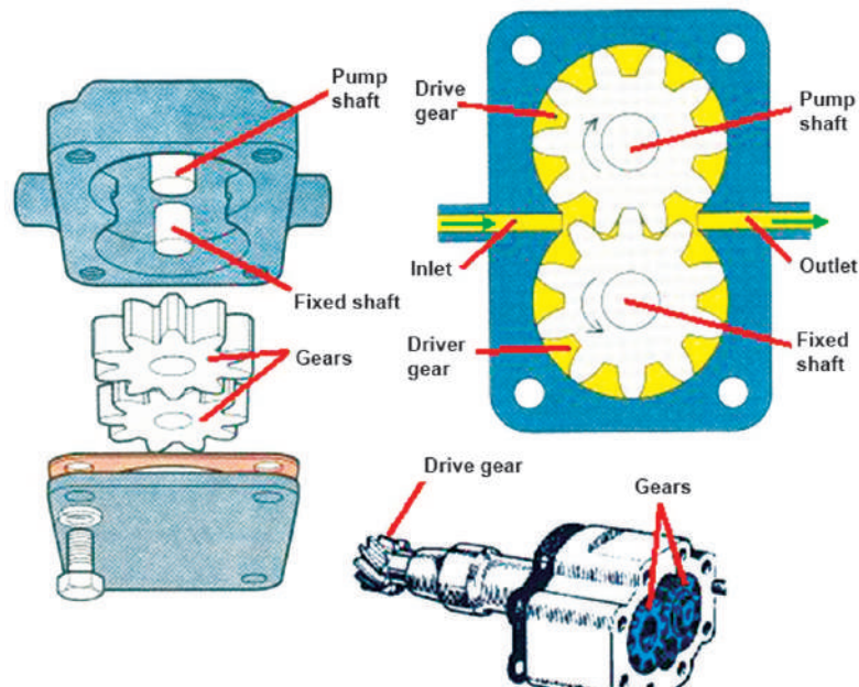
Fig. 2.1.4: Exploded view of gear type oil pump
