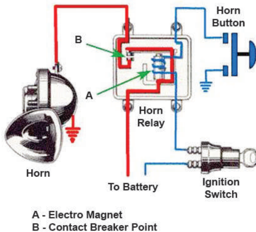
Fig.6.2.26: Horn Circuit of a Car.
