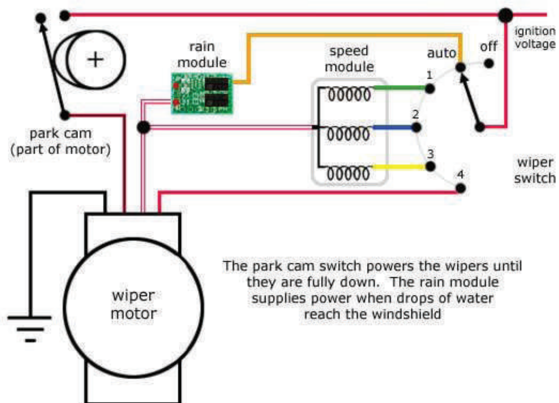
Fig.6.2.27: Wind Screen Wiper Circuit of a Car. (With rain module)
