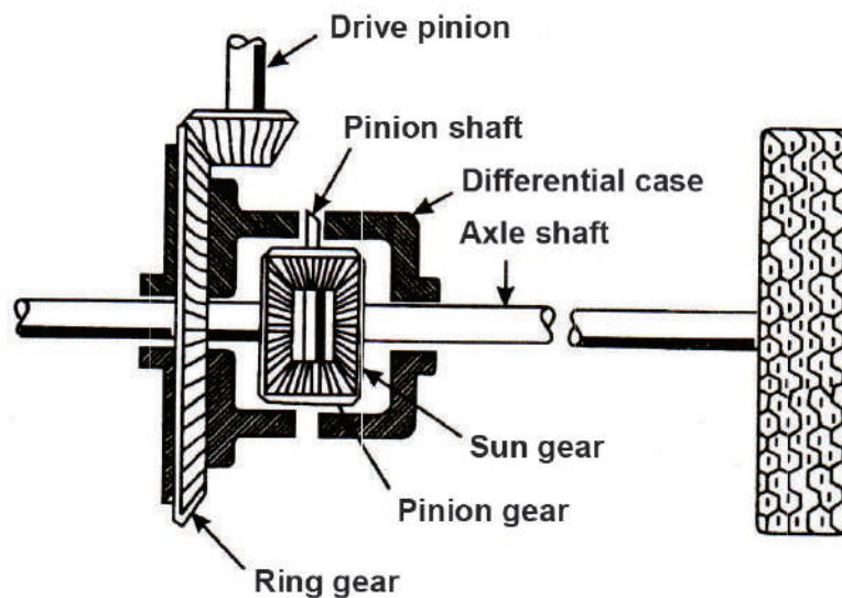
Fig.3.2.6: Differential Assembly.
