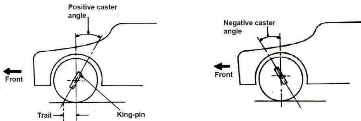
Fig. 4.2.4: Caster Angle
