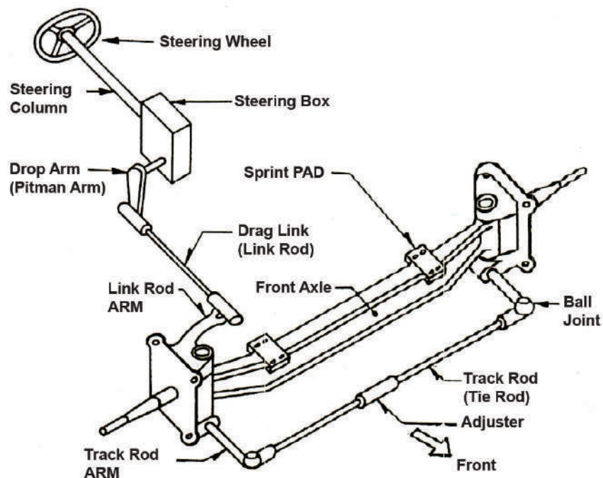
4.2.12: Steering Linkage for rigid axle suspension.
