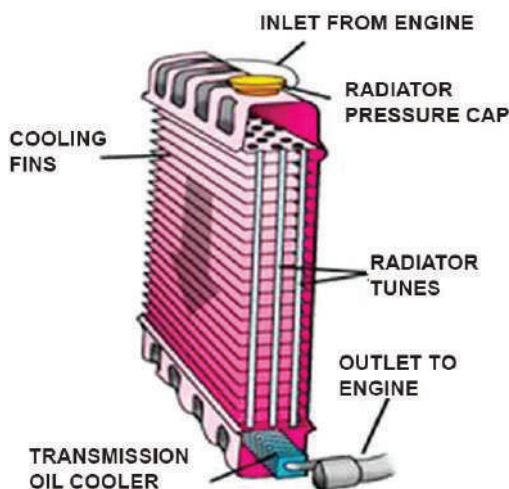
Fig.2.2.5: Radiator.
