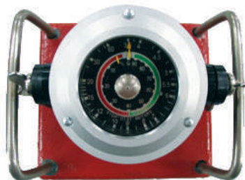
Fig. 1.1.20: Brake Efficiency Tester
