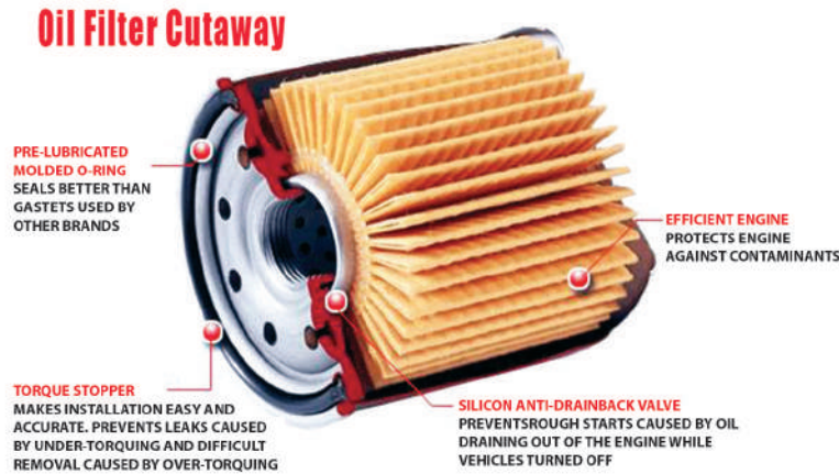
Fig. 2.1.7: Cut section view of a cartridge type oil filter
