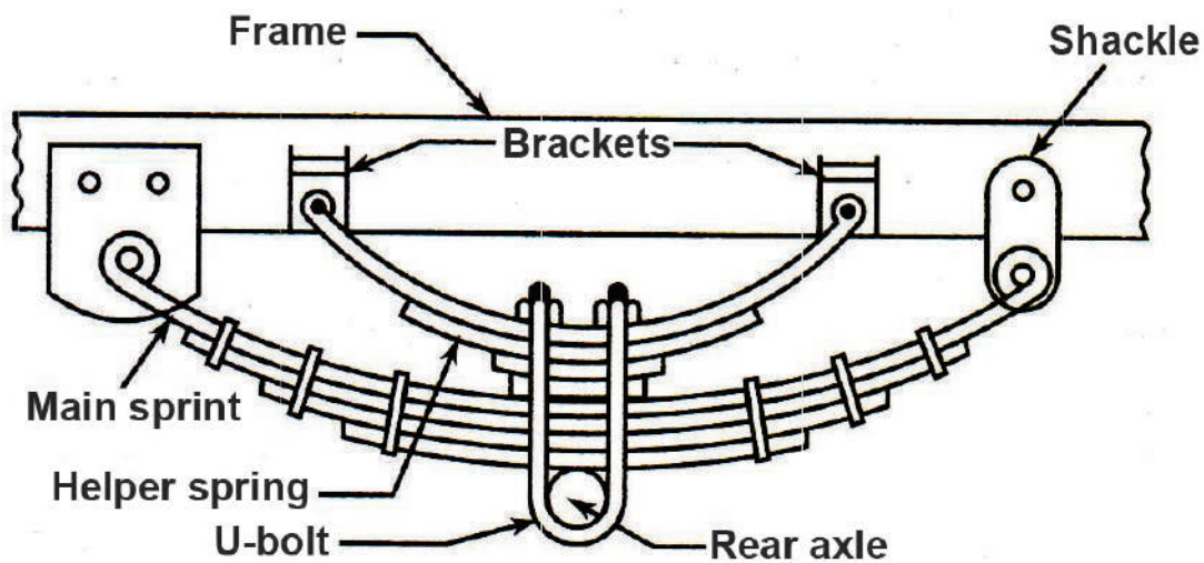
Fig.5.2.9: Helper Springs.
