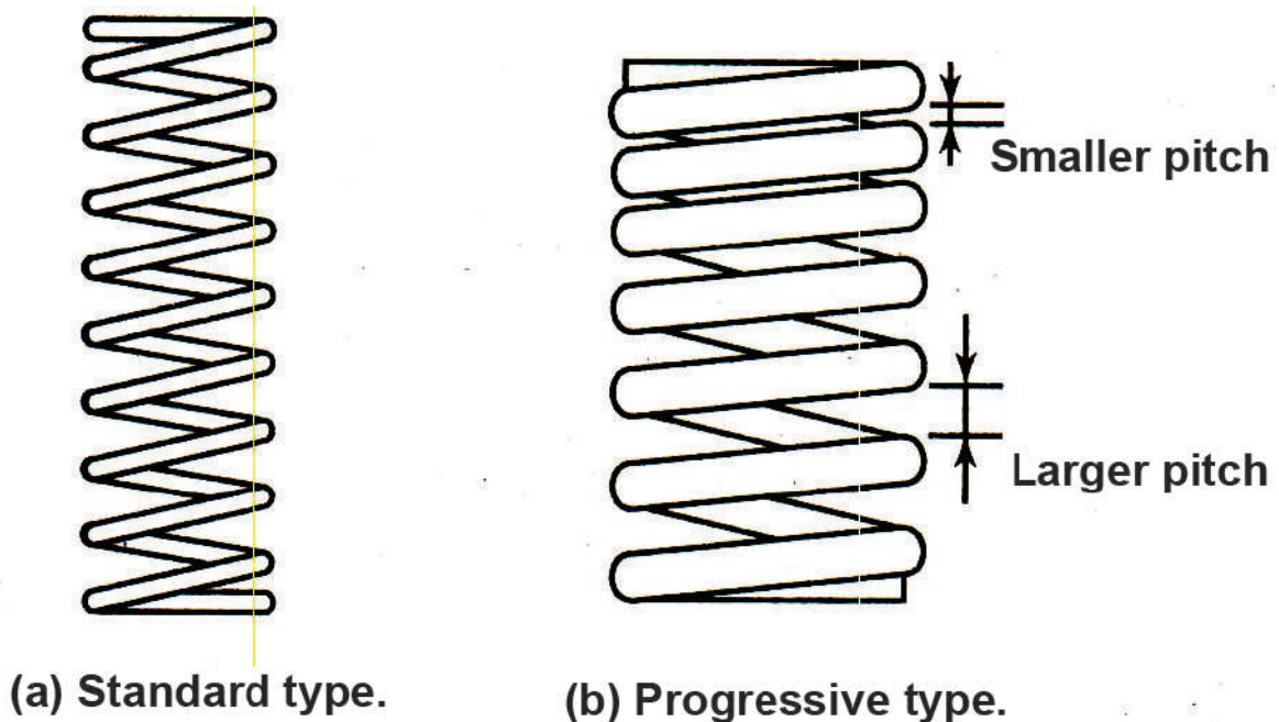
Fig.5.2.13: Coil Spring.
