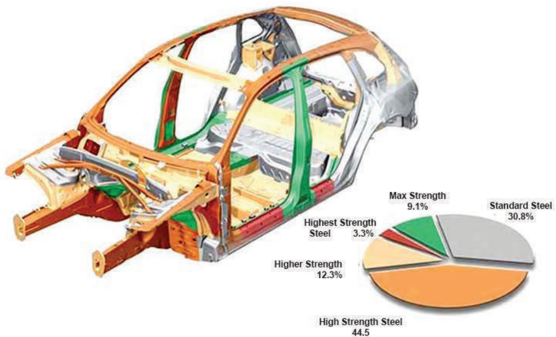
Fig.5.1.5: Frameless body Construction
